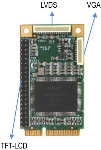
TFT-LCD (Optional)
